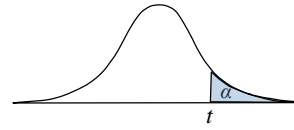
Right-tailed test
