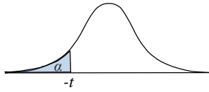
Left-tailed test
