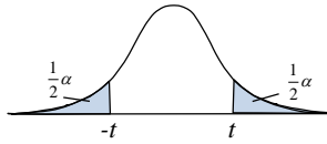
Two-tailed test
